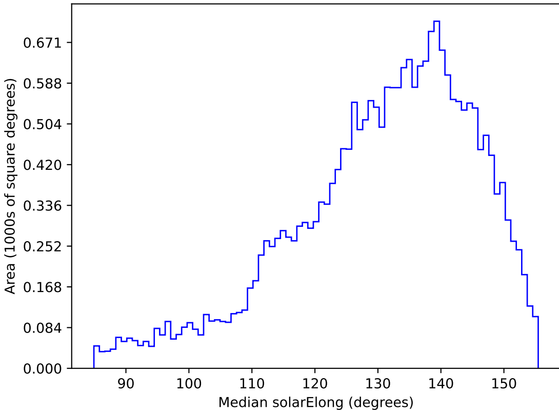
baseline_v3.2_10yrs All sky u band: Median solarElong
