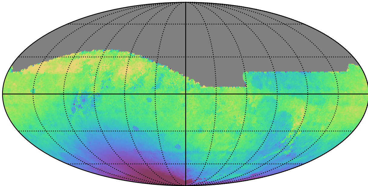
baseline_v3.2_10yrs All sky r band: Median solarElong
