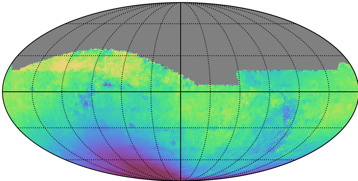
baseline_v3.2_10yrs All sky i band: Median solarElong
