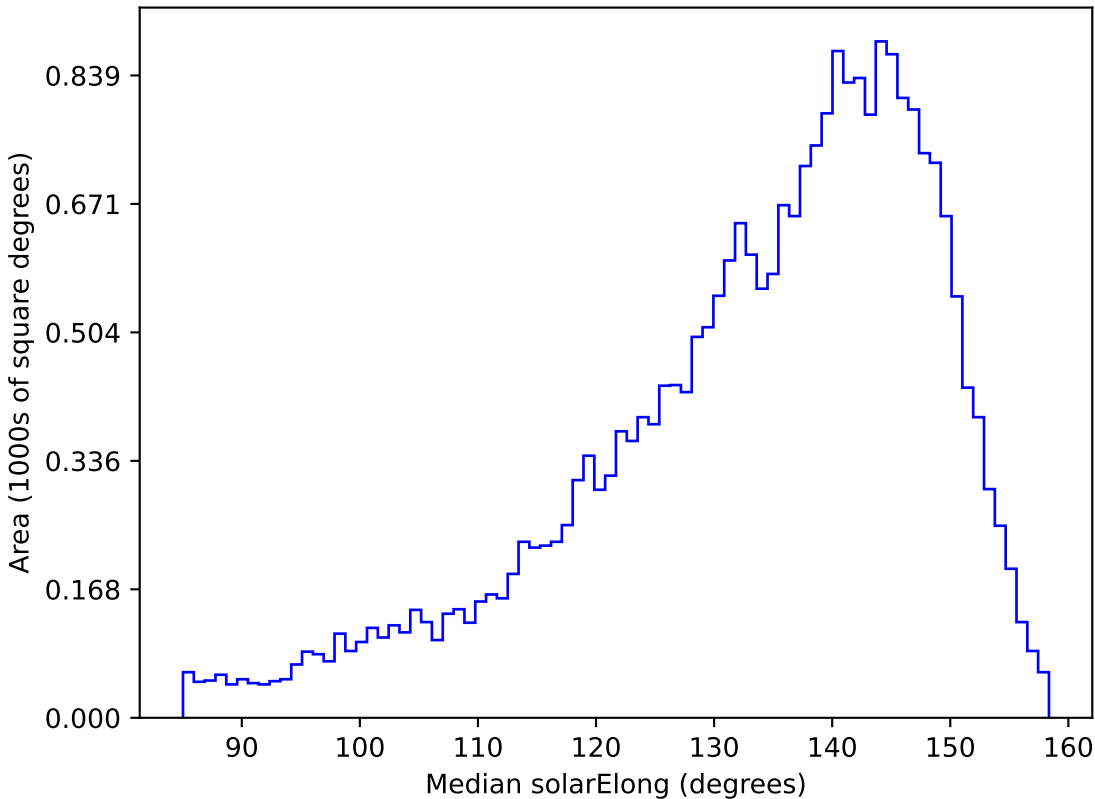
baseline_v3.2_10yrs All sky g band: Median solarElong
