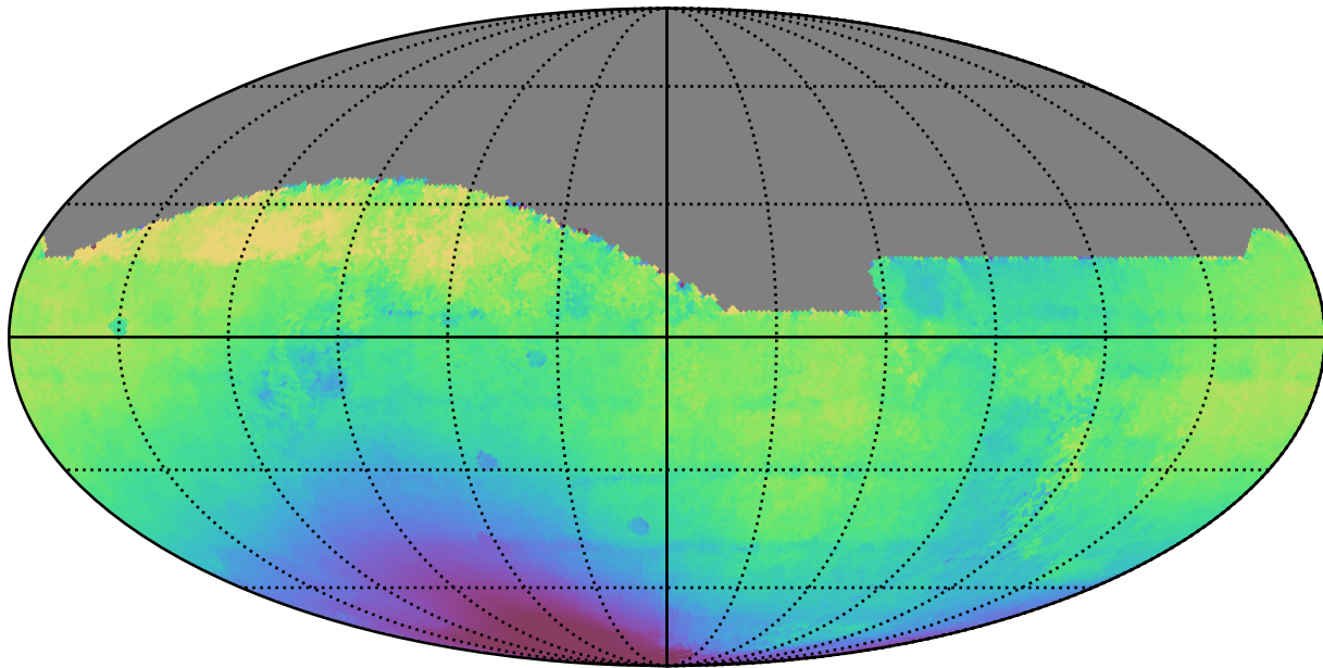
baseline_v3.2_10yrs All sky all bands: Median solarElong
