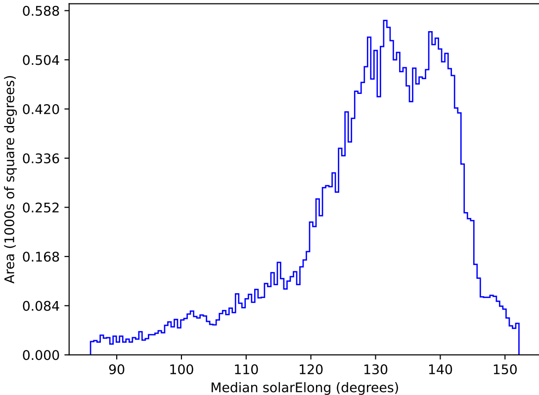
baseline_v3.2_10yrs All sky all bands: Median solarElong
