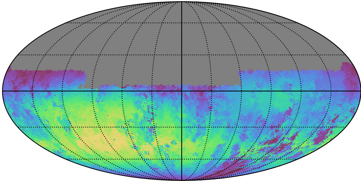
baseline_v3.2_10yrs Yr 1 u band: Median skyBrightness
