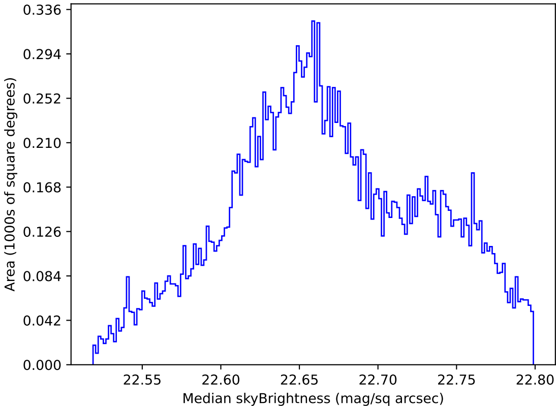
baseline_v3.2_10yrs Yr 1 u band: Median skyBrightness
