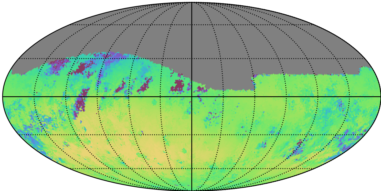
baseline_v3.2_10yrs Yr 1 r band: Median skyBrightness
