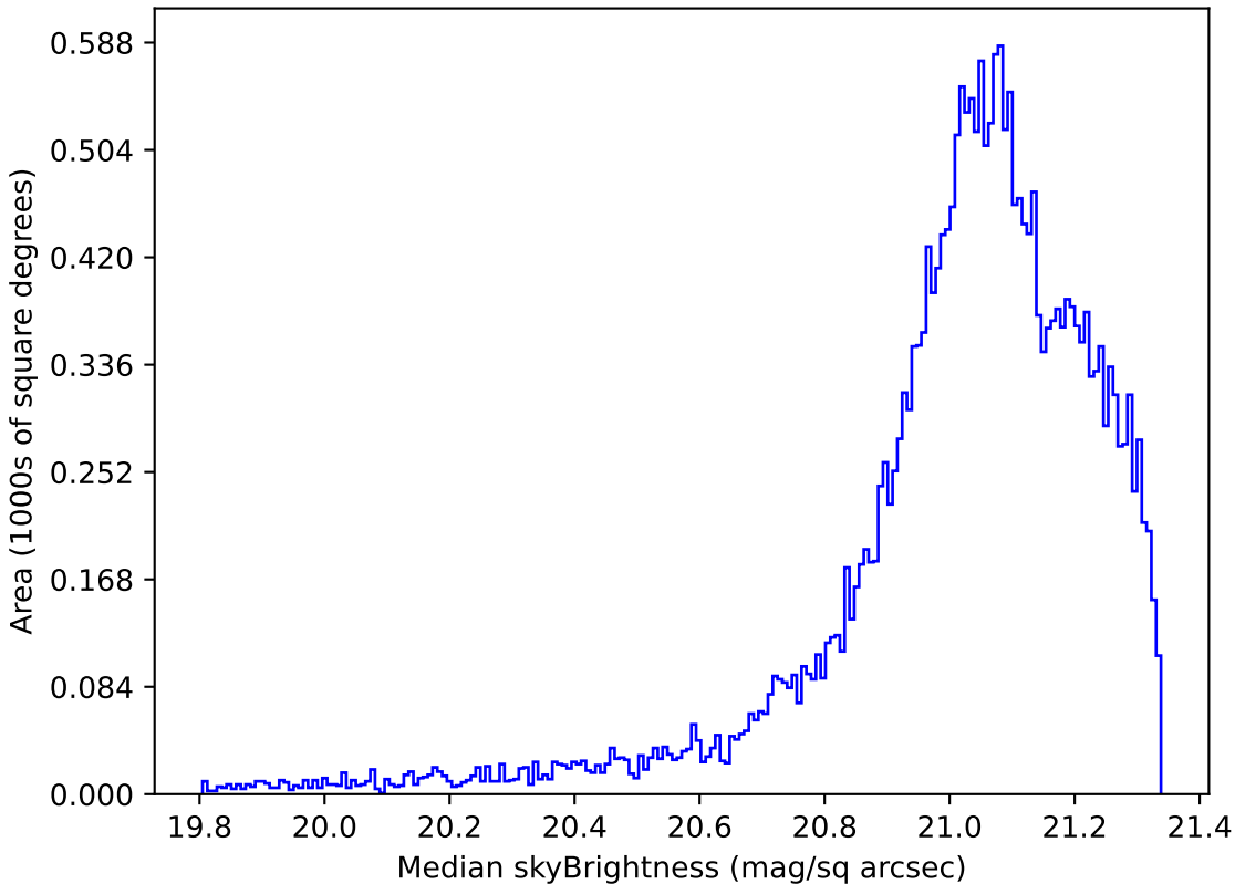
baseline_v3.2_10yrs Yr 1 r band: Median skyBrightness
