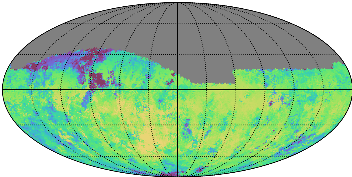
baseline_v3.2_10yrs Yr 1 i band: Median skyBrightness
