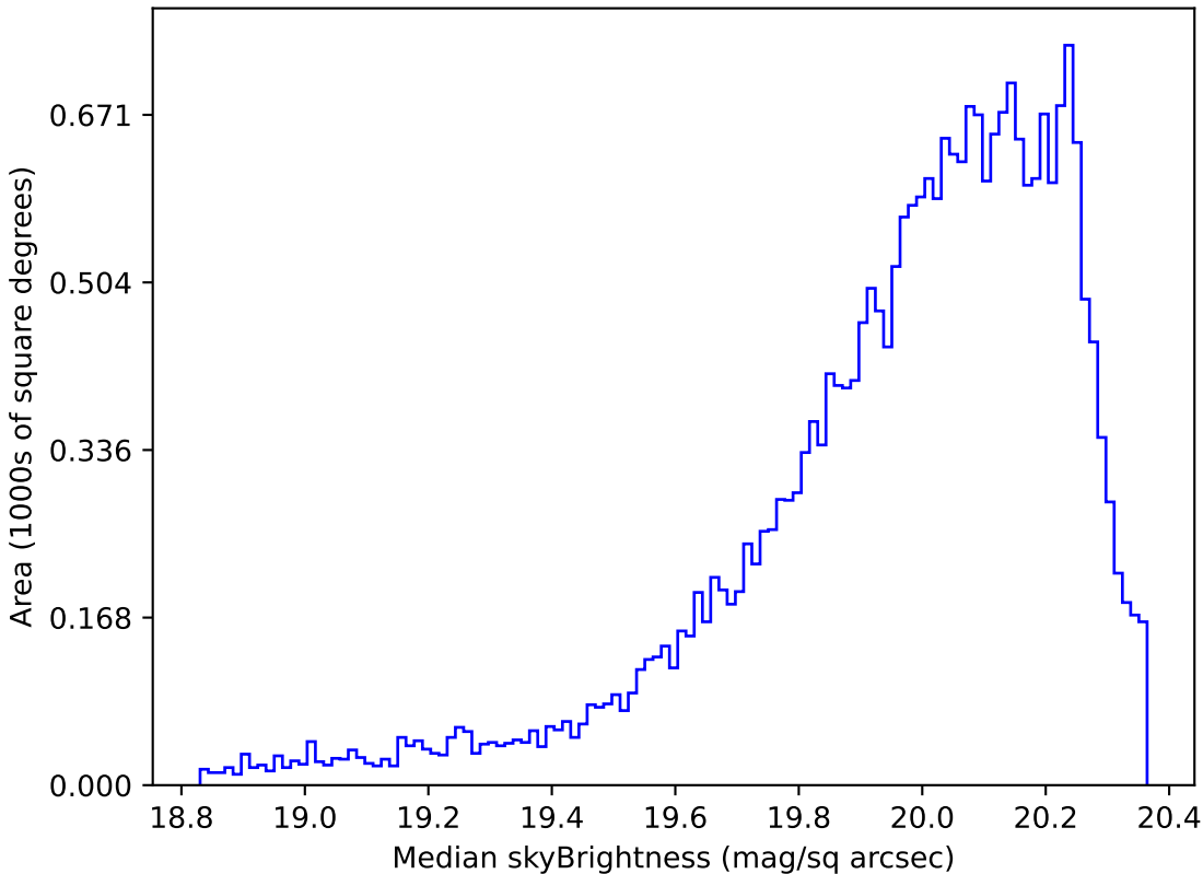
baseline_v3.2_10yrs Yr 1 i band: Median skyBrightness
