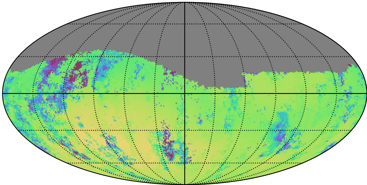
baseline_v3.2_10yrs Yr 1 g band: Median skyBrightness
