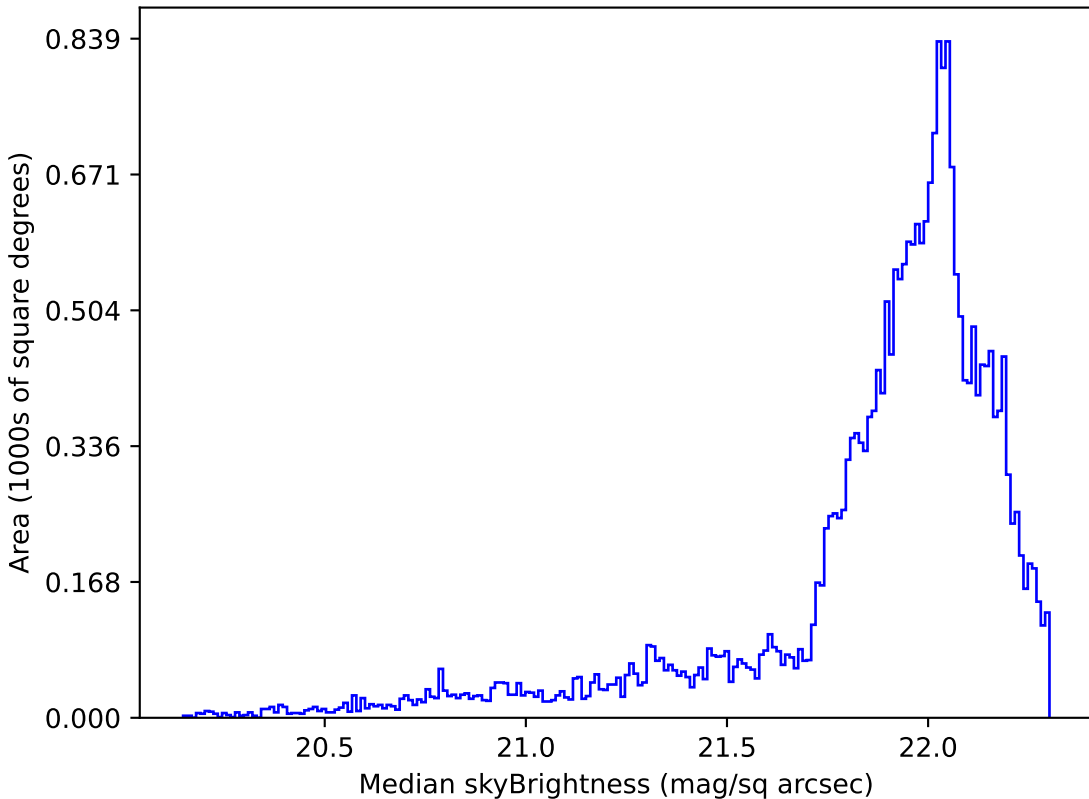
baseline_v3.2_10yrs Yr 1 g band: Median skyBrightness
