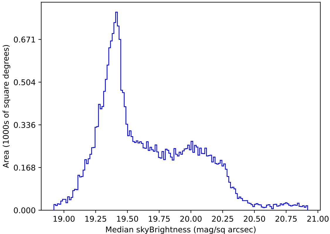
baseline_v3.2_10yrs Yr 1 all bands: Median skyBrightness
