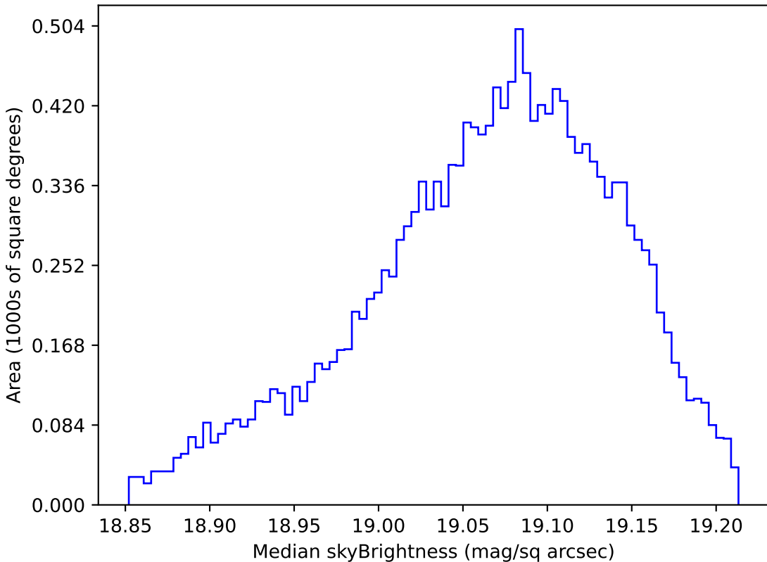
baseline_v3.2_10yrs WFD z band: Median skyBrightness
