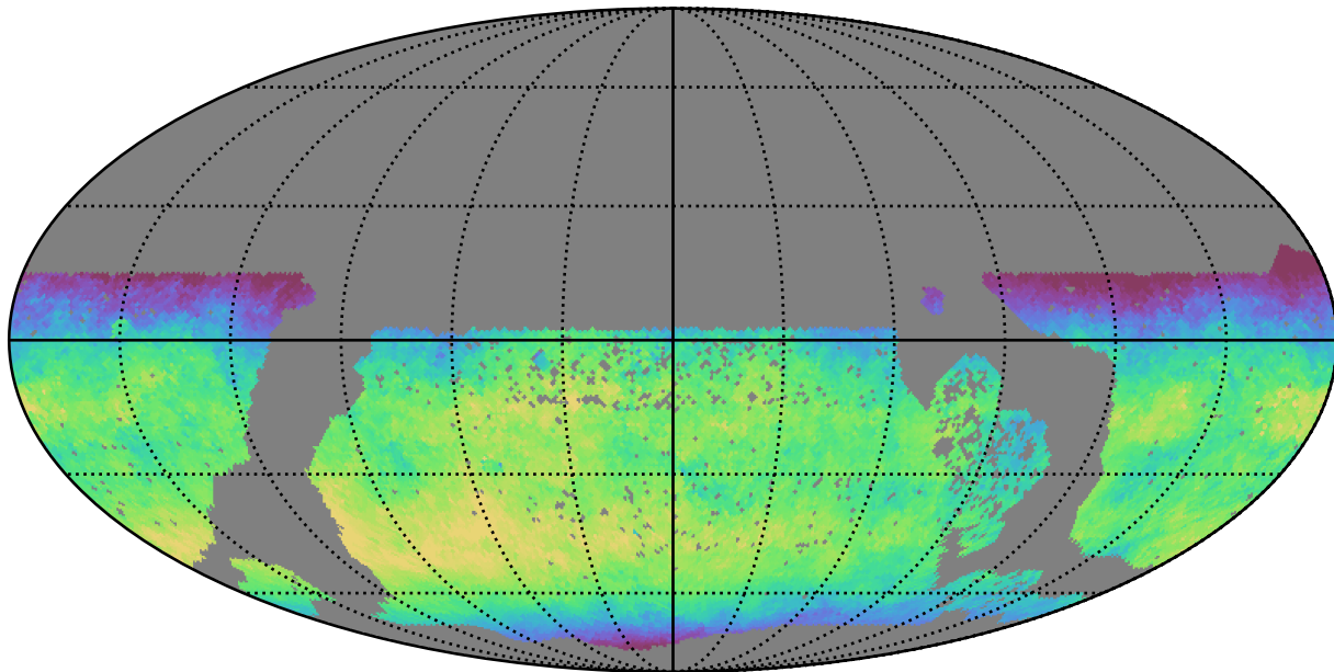
baseline_v3.2_10yrs WFD y band: Median skyBrightness
