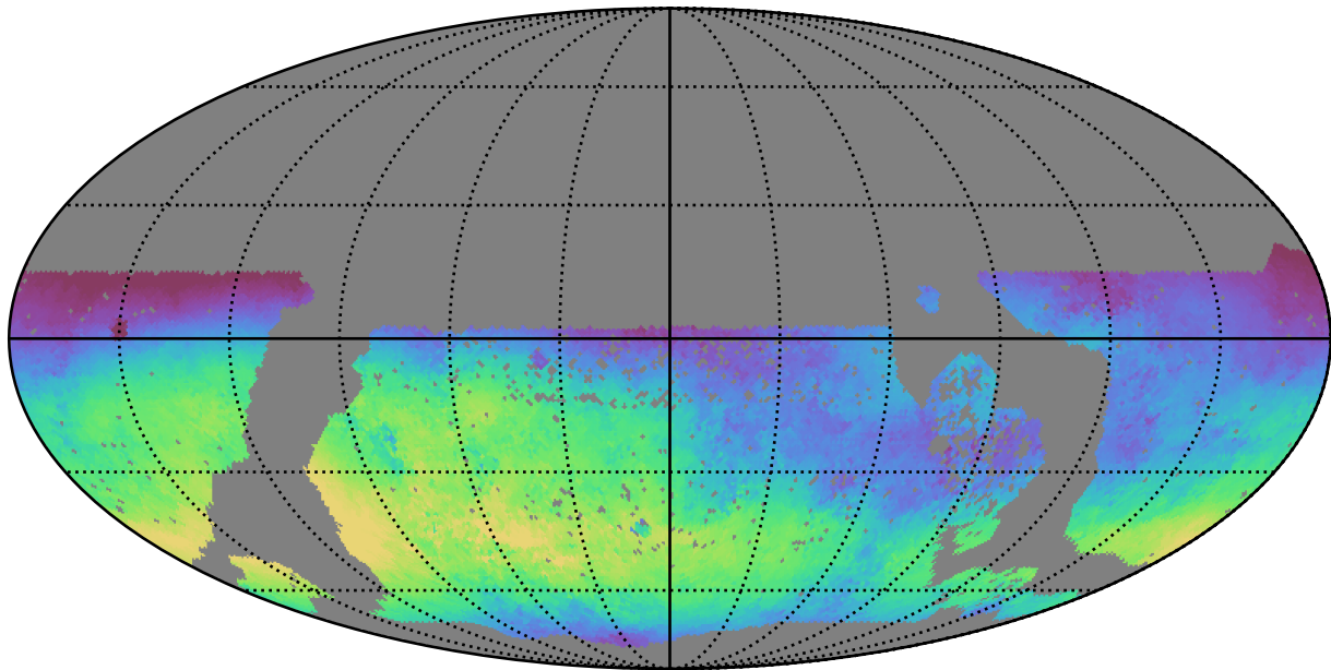
baseline_v3.2_10yrs WFD u band: Median skyBrightness
