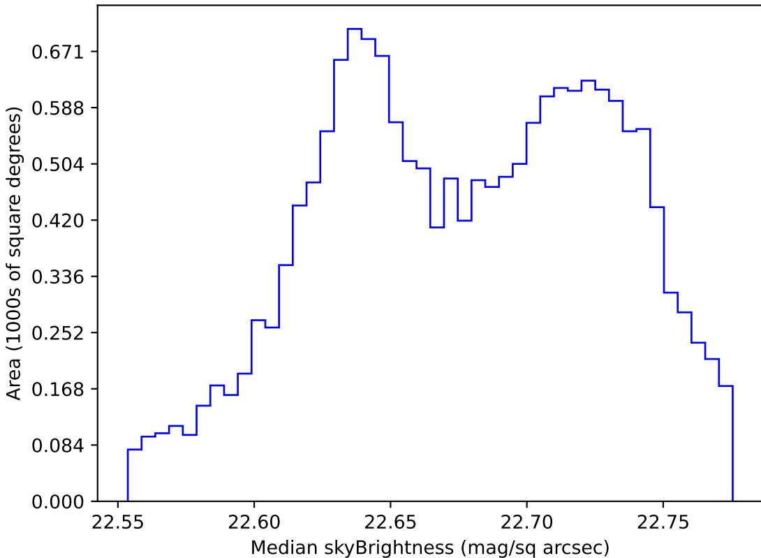
baseline_v3.2_10yrs WFD u band: Median skyBrightness
