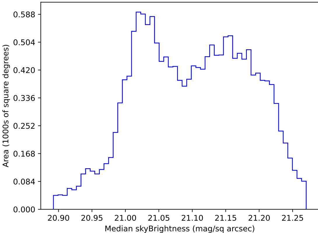
baseline_v3.2_10yrs WFD r band: Median skyBrightness
