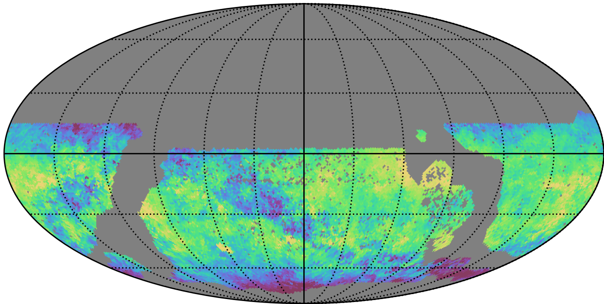
baseline_v3.2_10yrs WFD i band: Median skyBrightness
