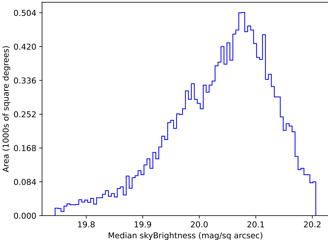
baseline_v3.2_10yrs WFD i band: Median skyBrightness
