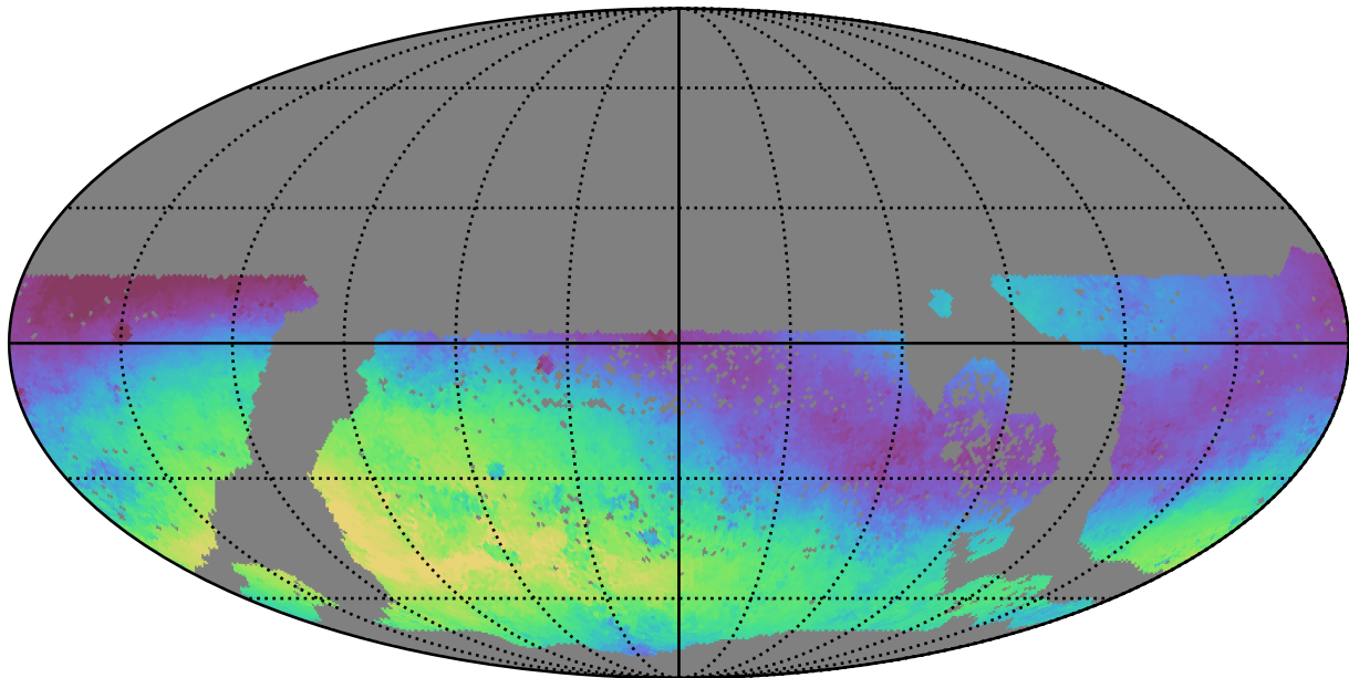
baseline_v3.2_10yrs WFD g band: Median skyBrightness
