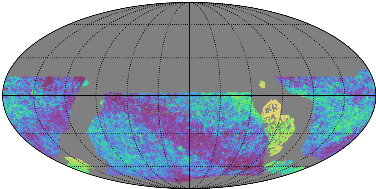
baseline_v3.2_10yrs WFD all bands: Median skyBrightness
