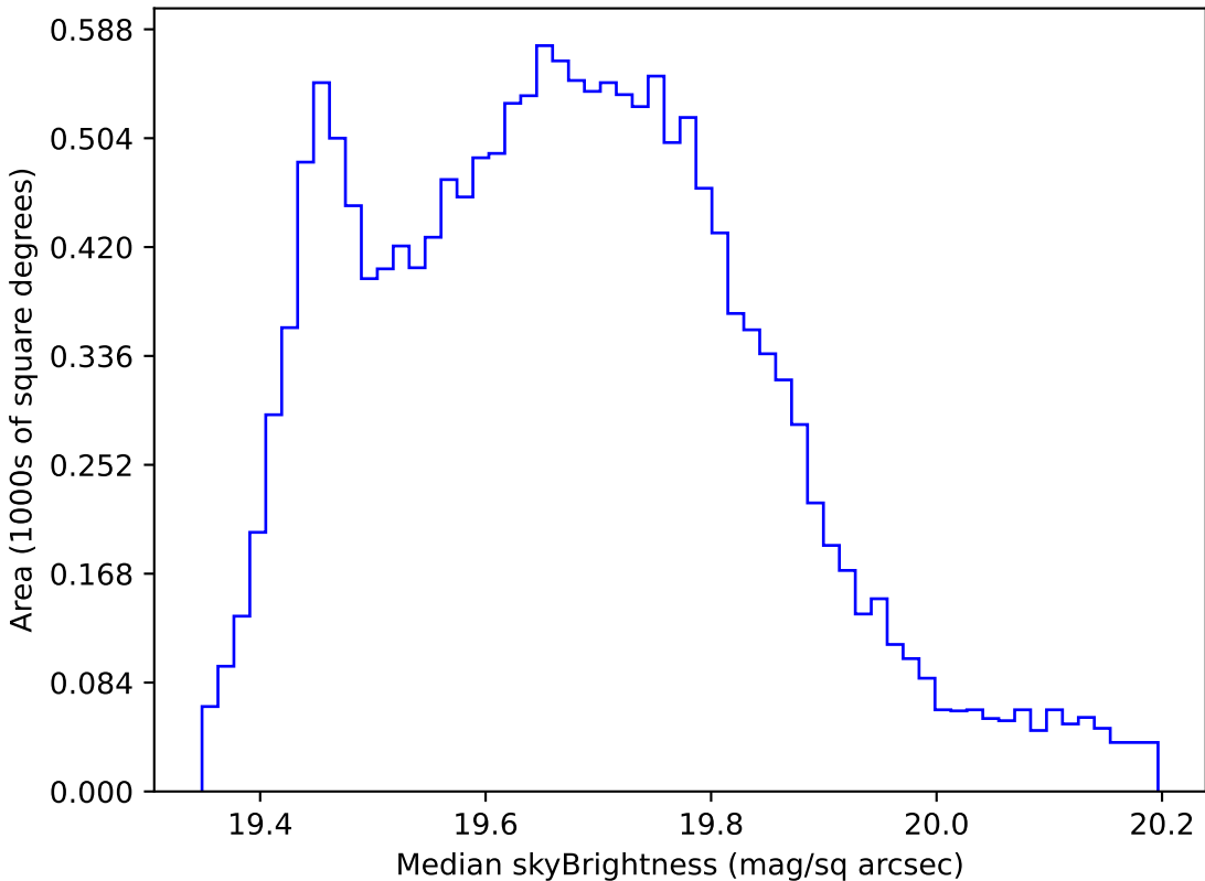
baseline_v3.2_10yrs WFD all bands: Median skyBrightness
