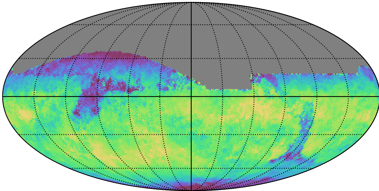
baseline_v3.2_10yrs All sky z band: Median skyBrightness
