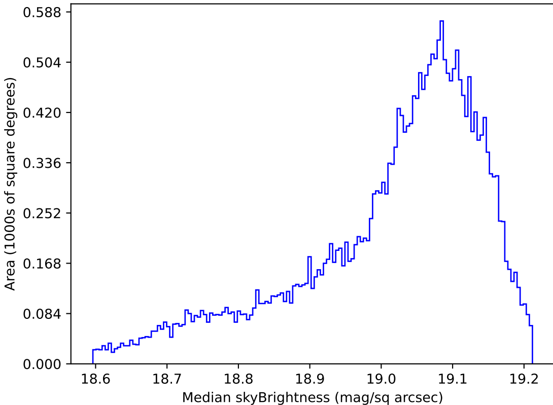
baseline_v3.2_10yrs All sky z band: Median skyBrightness
