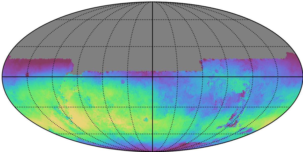
baseline_v3.2_10yrs All sky u band: Median skyBrightness
