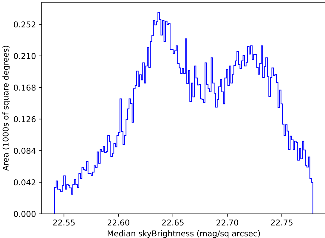
baseline_v3.2_10yrs All sky u band: Median skyBrightness
