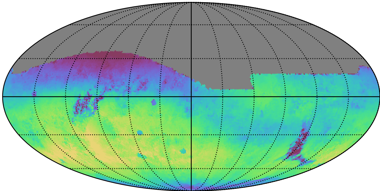
baseline_v3.2_10yrs All sky r band: Median skyBrightness
