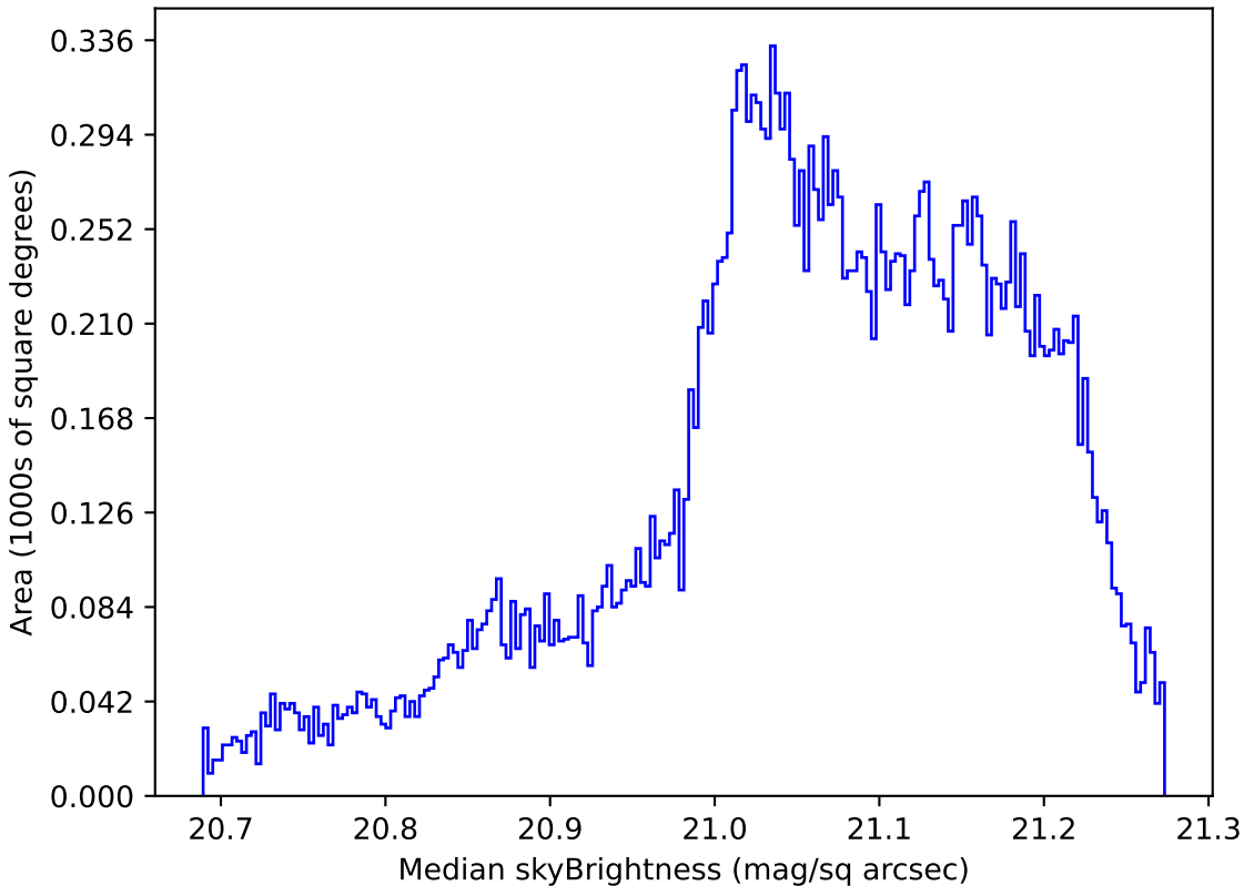
baseline_v3.2_10yrs All sky r band: Median skyBrightness
