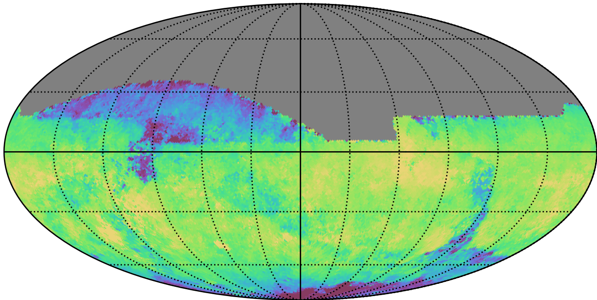
baseline_v3.2_10yrs All sky i band: Median skyBrightness
