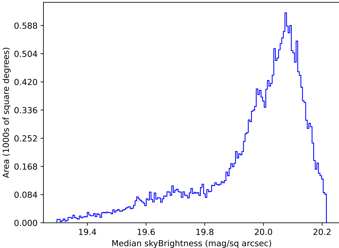
baseline_v3.2_10yrs All sky i band: Median skyBrightness
