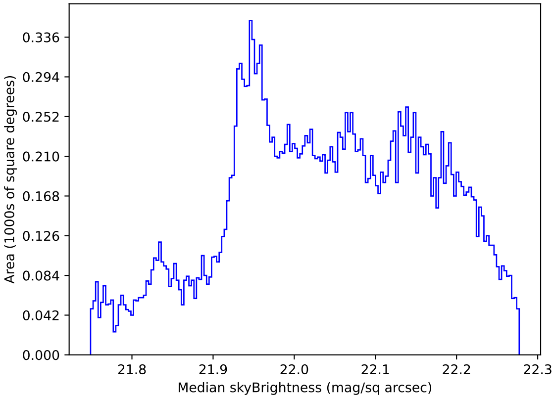
baseline_v3.2_10yrs All sky g band: Median skyBrightness
