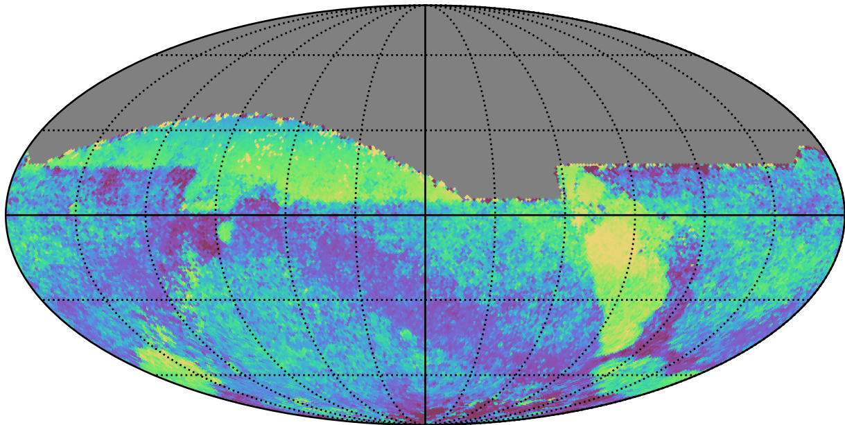
baseline_v3.2_10yrs All sky all bands: Median skyBrightness
