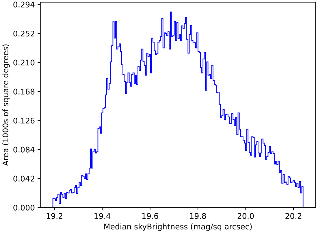
baseline_v3.2_10yrs All sky all bands: Median skyBrightness
