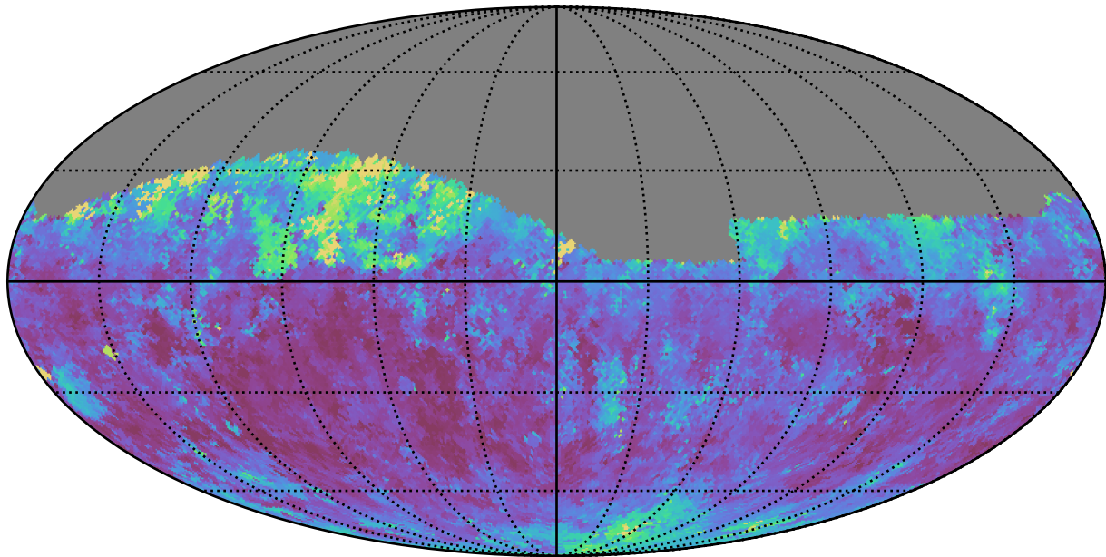
baseline_v3.2_10yrs Yr 1 z band: Median seeingGeom
