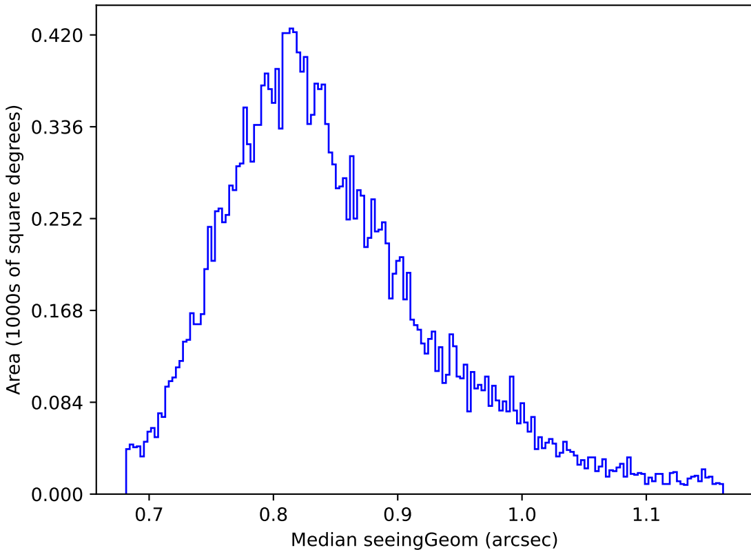
baseline_v3.2_10yrs Yr 1 y band: Median seeingGeom
