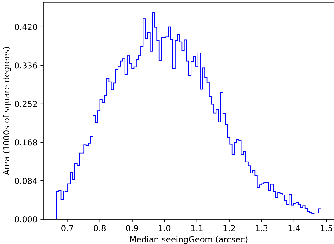
baseline_v3.2_10yrs Yr 1 u band: Median seeingGeom
