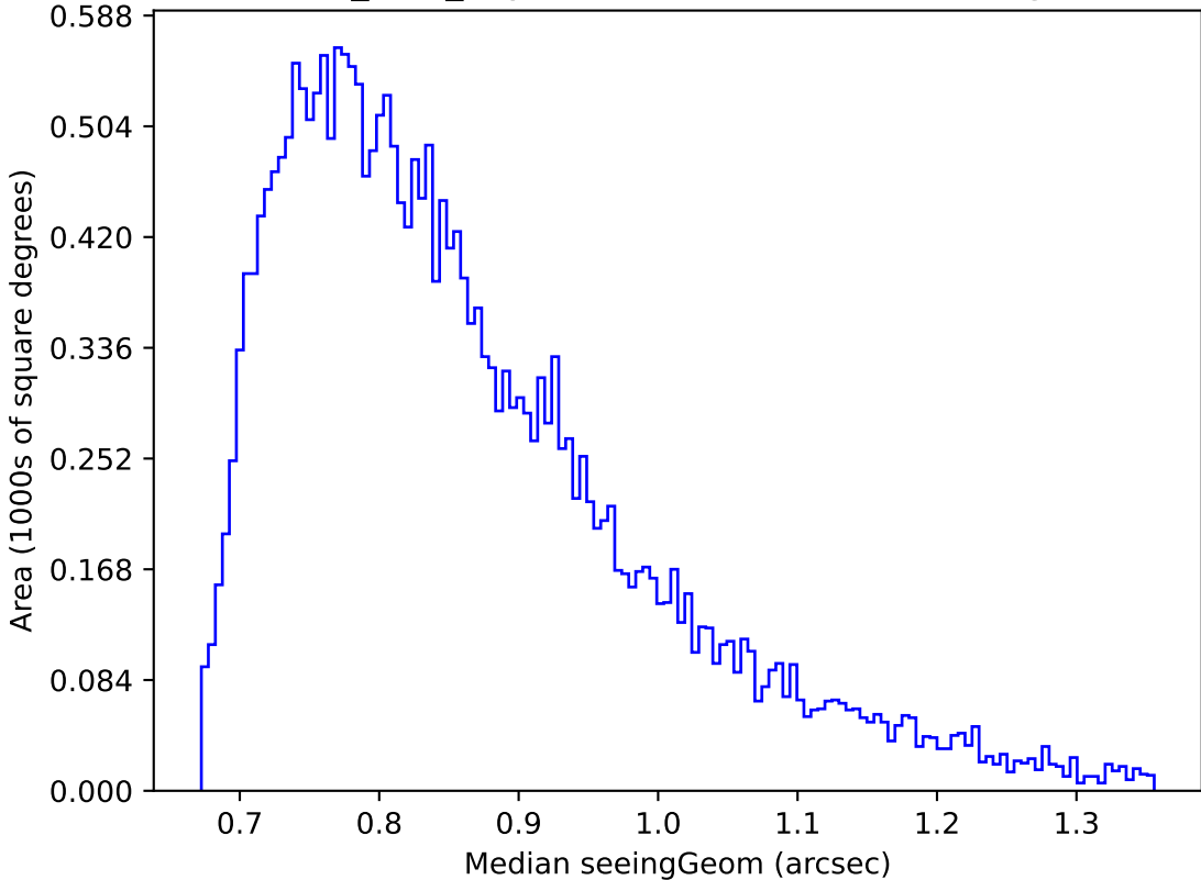
baseline_v3.2_10yrs Yr 1 r band: Median seeingGeom
