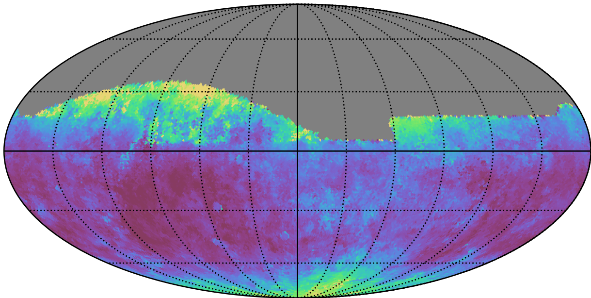
baseline_v3.2_10yrs Yr 1 all bands: Median seeingGeom
