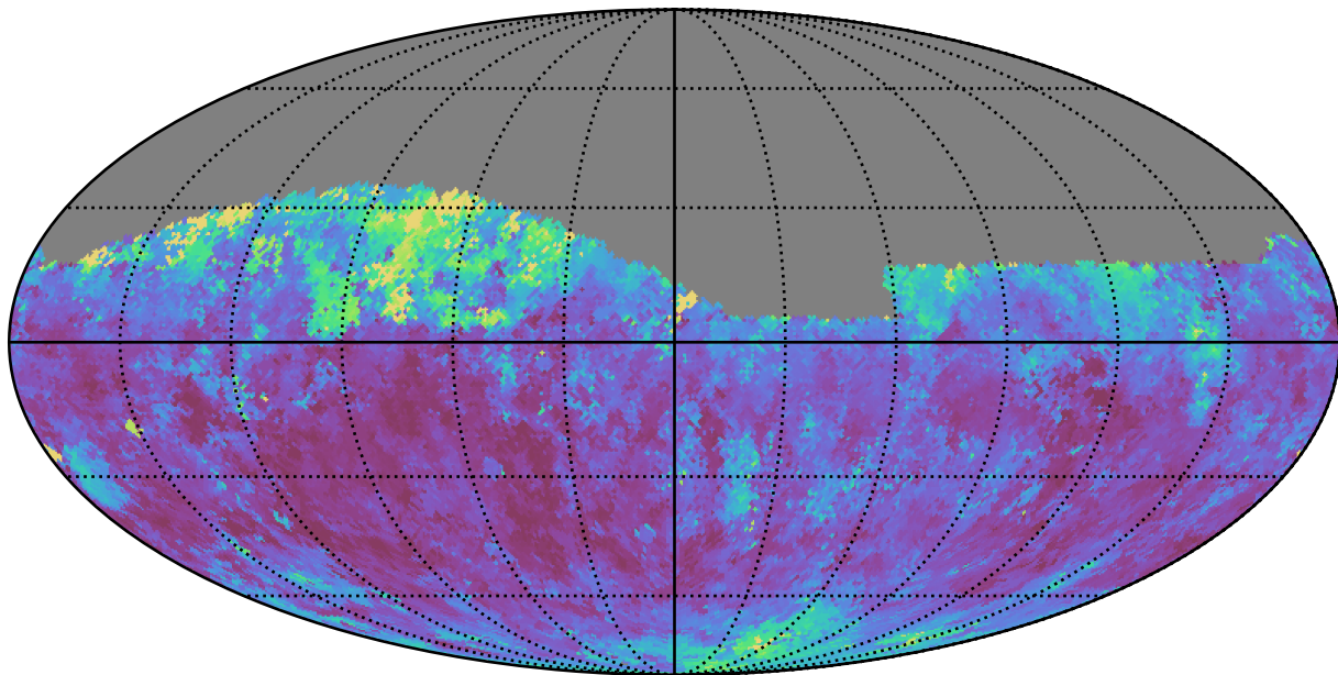
baseline_v3.2_10yrs Yr 1 z band: Median seeingEff
