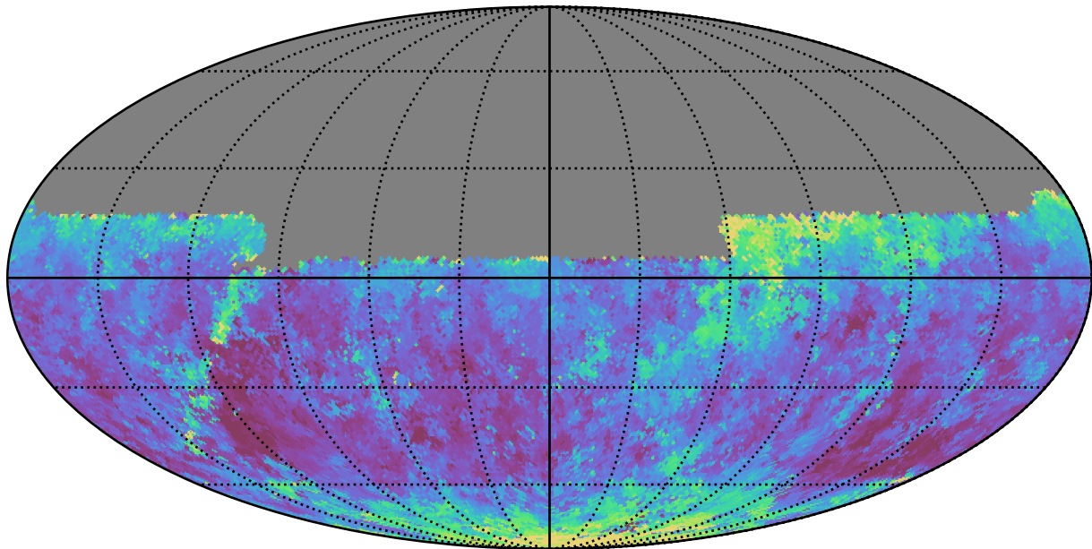
baseline_v3.2_10yrs Yr 1 y band: Median seeingEff
