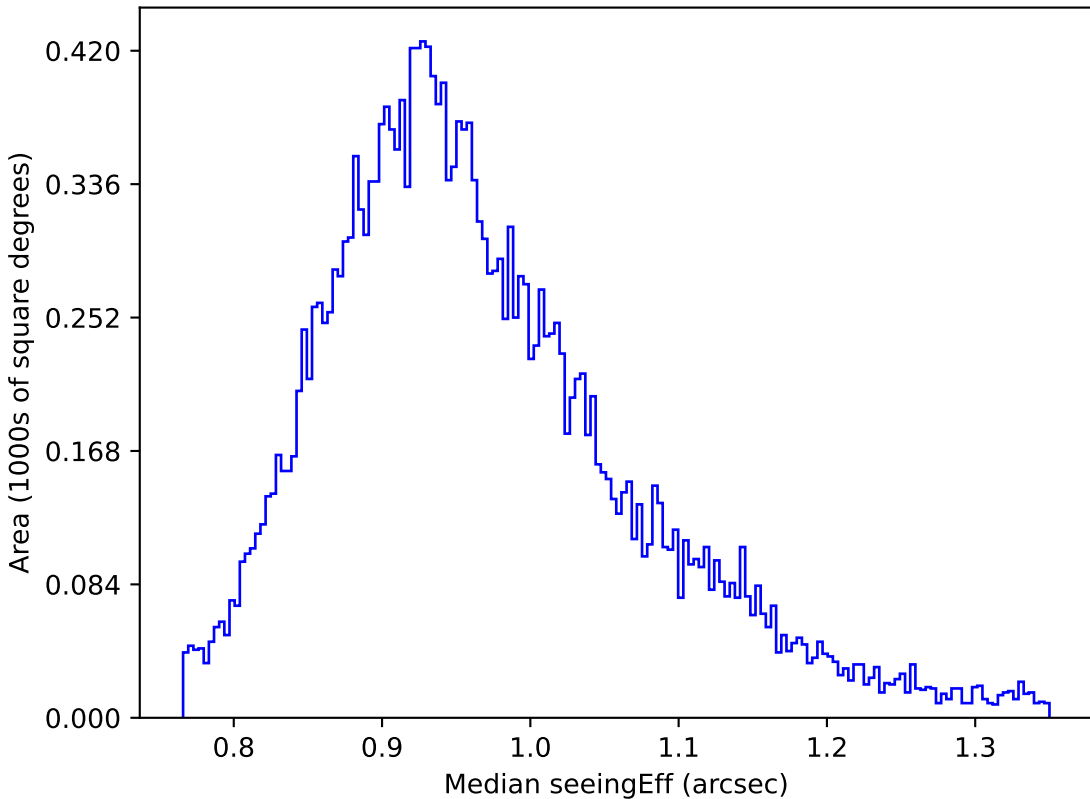
baseline_v3.2_10yrs Yr 1 y band: Median seeingEff
