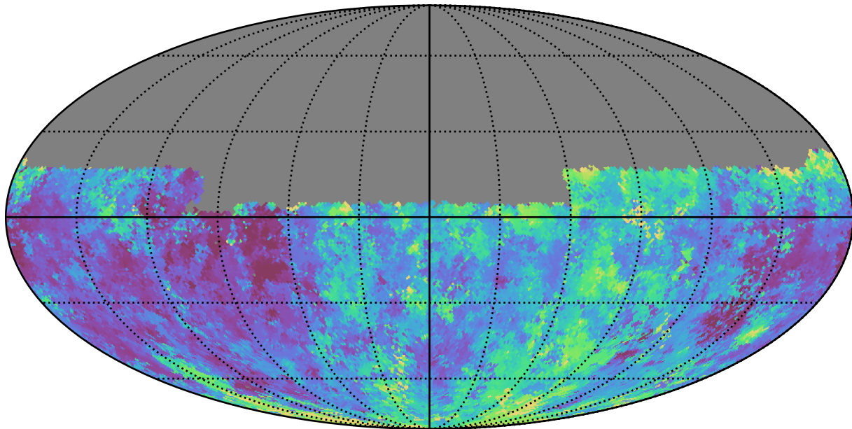
baseline_v3.2_10yrs Yr 1 u band: Median seeingEff
