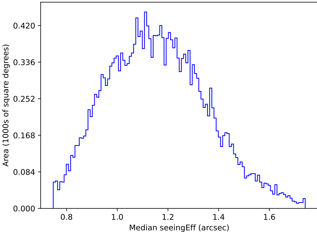
baseline_v3.2_10yrs Yr 1 u band: Median seeingEff
