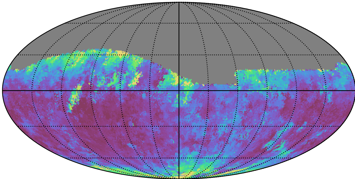
baseline_v3.2_10yrs Yr 1 r band: Median seeingEff
