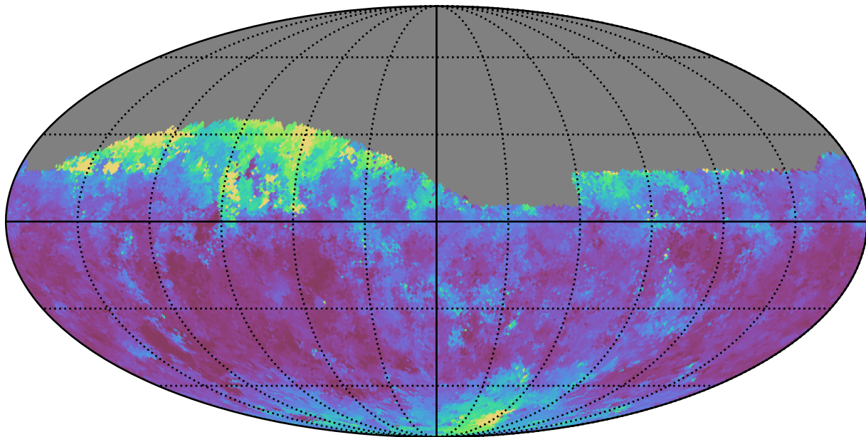
baseline_v3.2_10yrs Yr 1 i band: Median seeingEff
