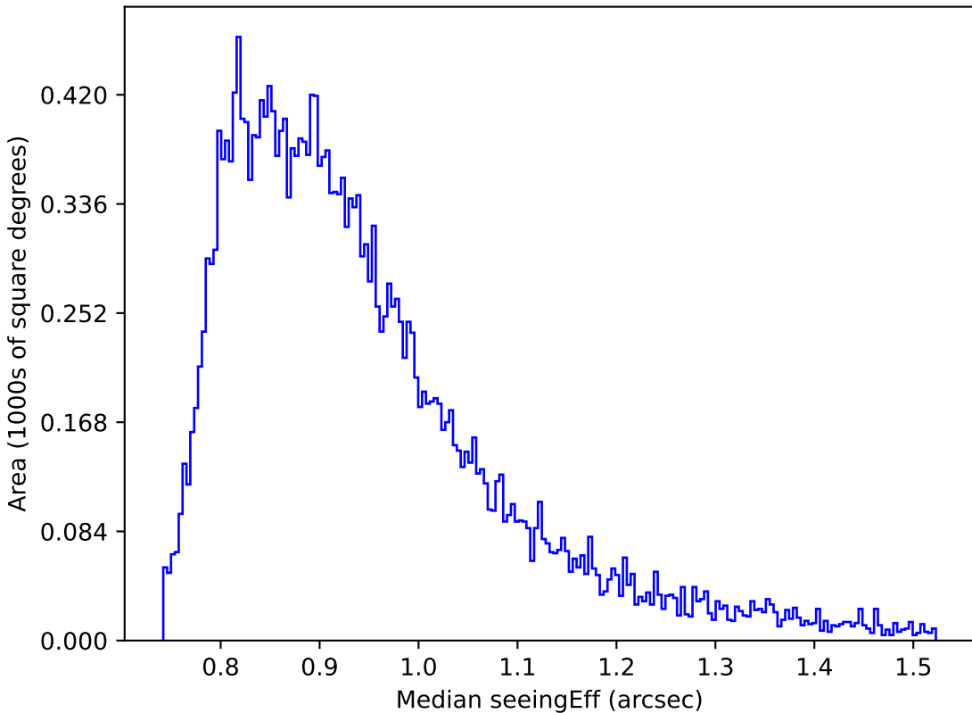
baseline_v3.2_10yrs Yr 1 i band: Median seeingEff
