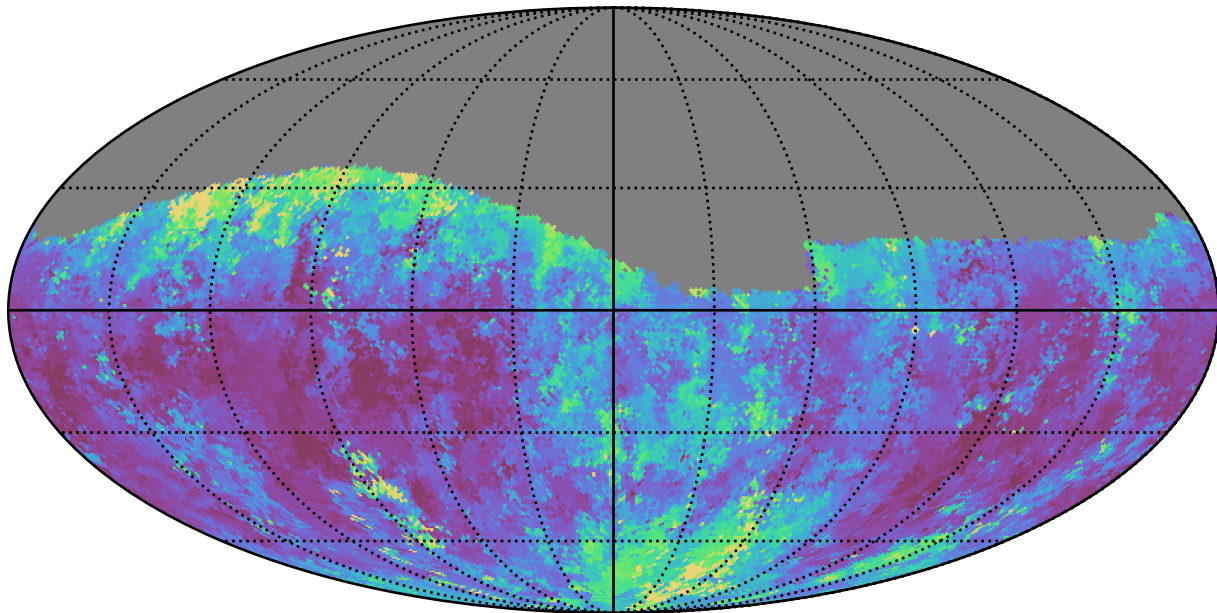
baseline_v3.2_10yrs Yr 1 g band: Median seeingEff
